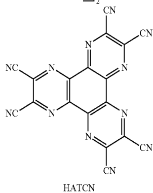
HATCN
