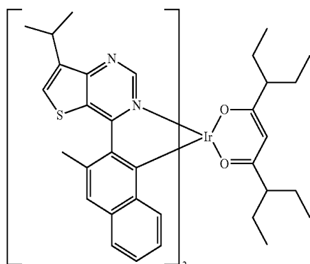
Compound 6,040
