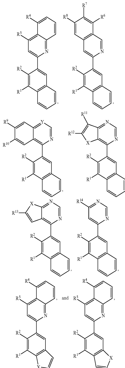
Formula I
